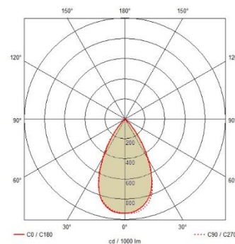
CHILL60 LED
