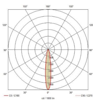
CHILL18 LED
