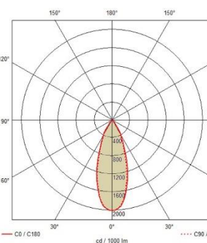
CHILL36 LED
