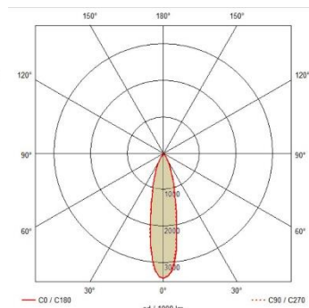
CHILL24 LED
