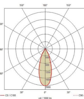
CHILL36 LED
